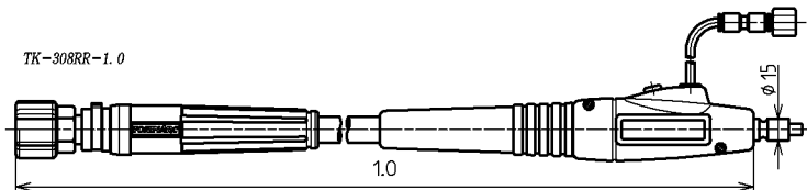
TK-308RR-1.0-SC
