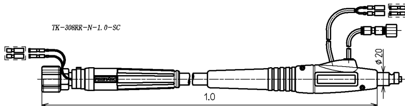
TK-308RR-D-1.0
