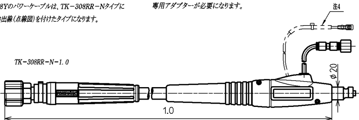
TK-308RR-N-1.0-SC
